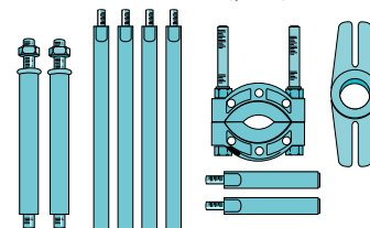
Part No. 19320100 (p.37)
